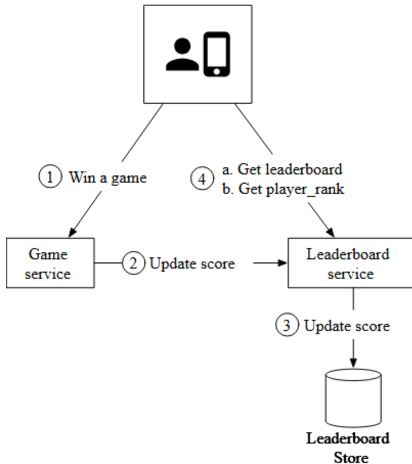
Figure 2 High-level design
