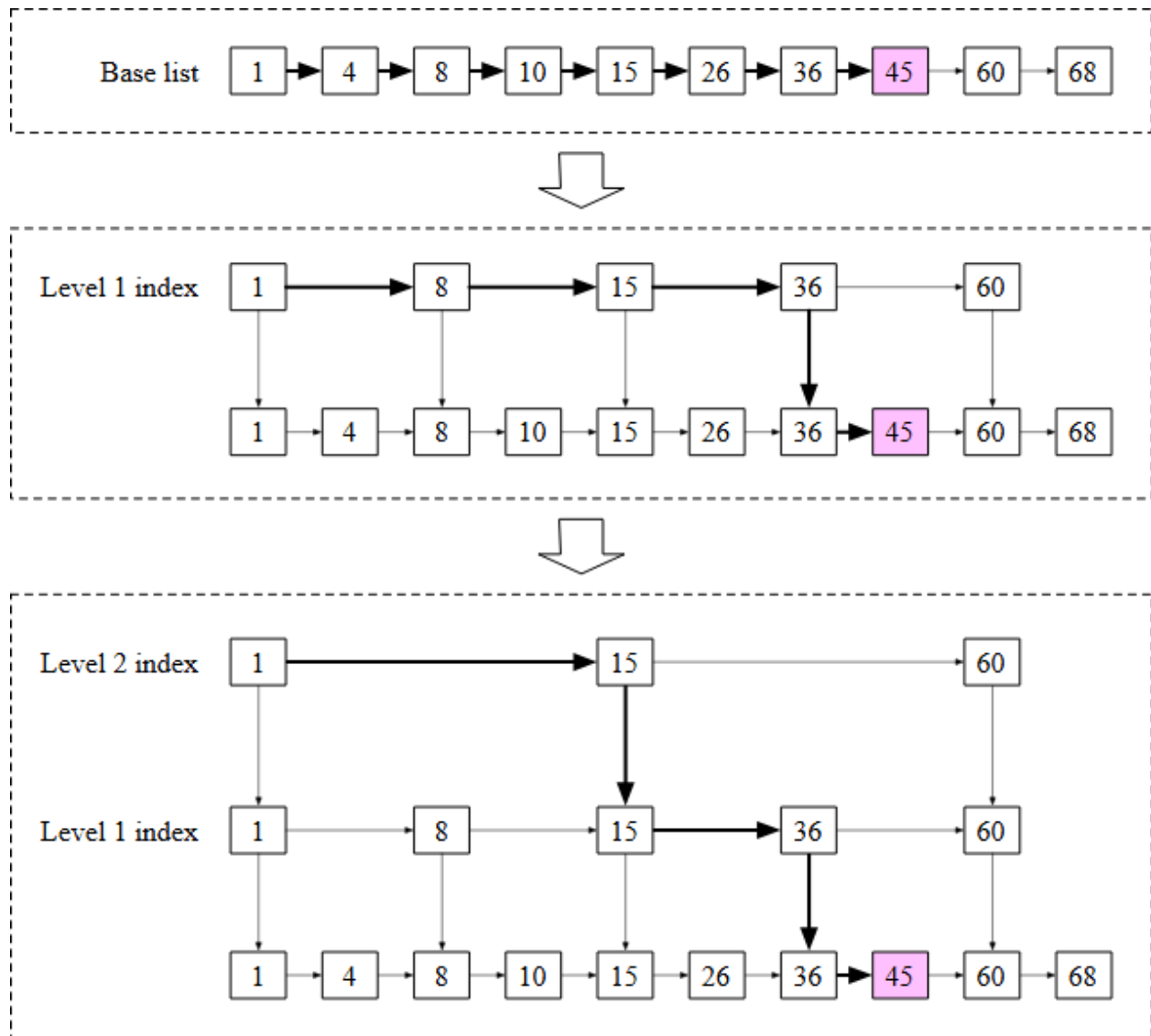
Figure 9 Skip list
