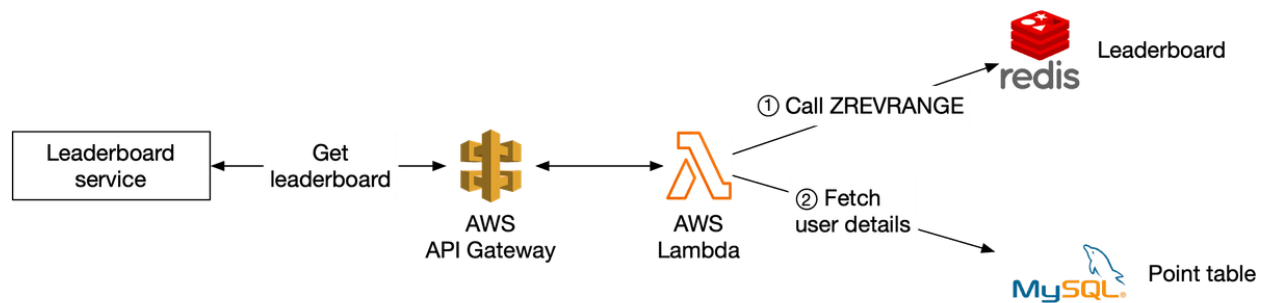
Figure 17 Retrieve leaderboard
