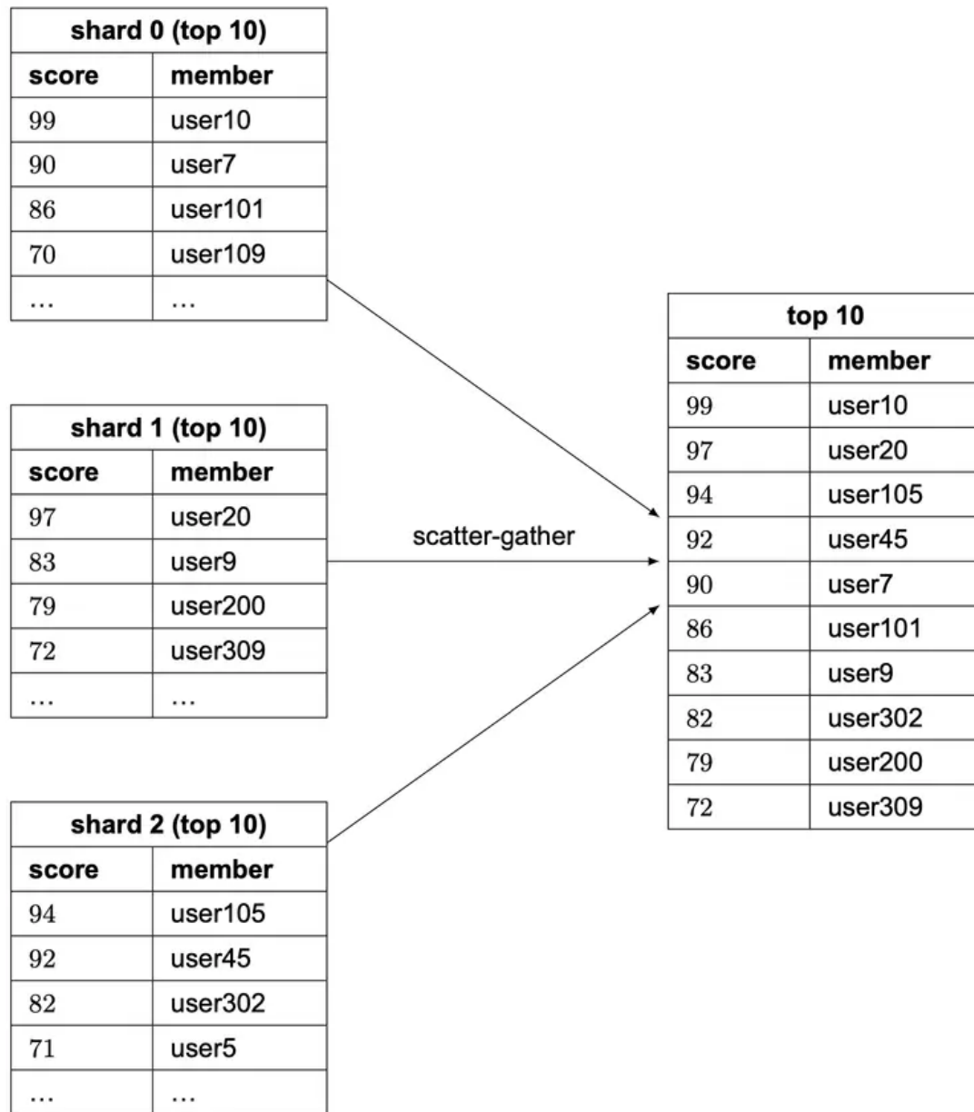
Figure 20 Scatter-gather
