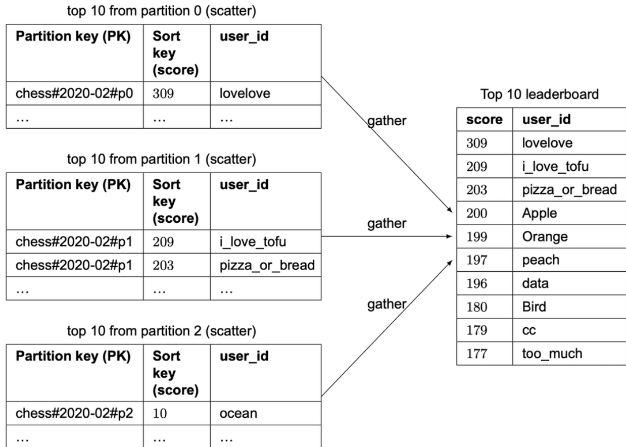
Figure 25 Scatter-gather
