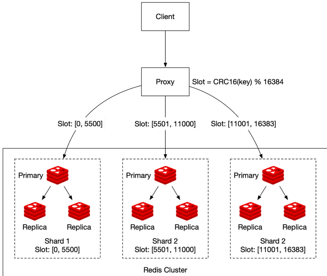
Figure 19 Hash partition
